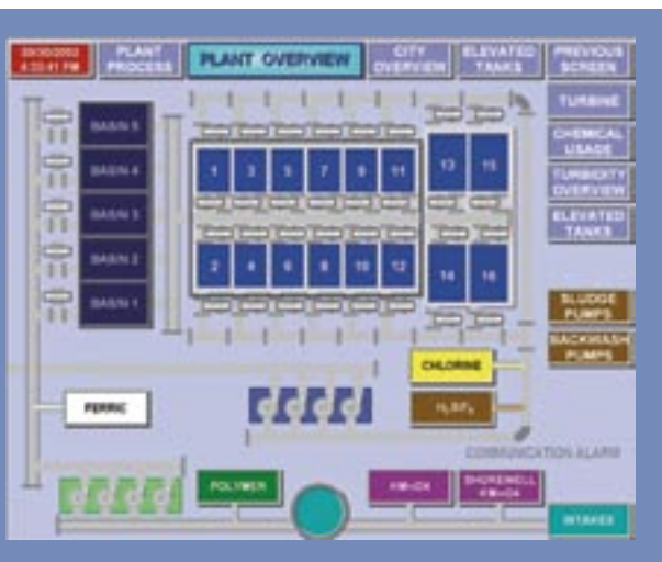
Plant Overview Screen at Racine Water
